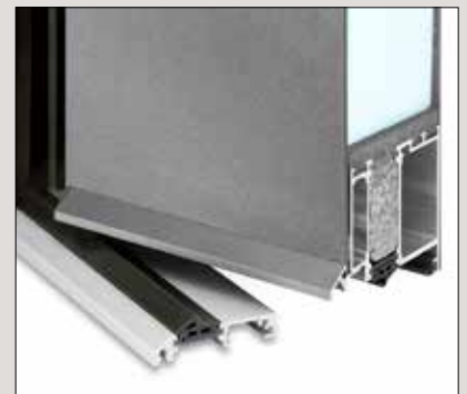
Weather bar Deverts water away from door sill.
